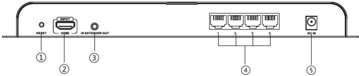
Figure 1: Transmitter (TX) - Back Panel
