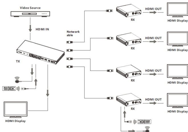
Figure 4: Application Diagram
